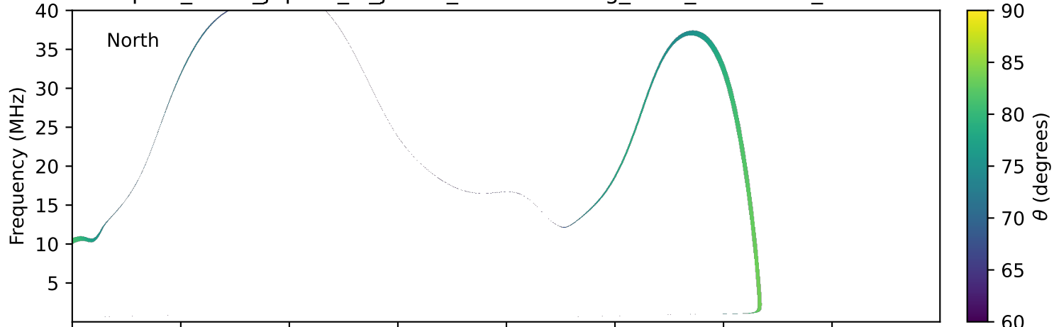
expres_earth_jupiter_io_jrm33_lossc-wid1deg_3kev_20261108_v11.cdf
