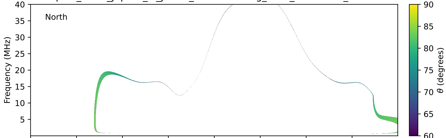
expres_earth_jupiter_io_jrm33_lossc-wid1deg_3kev_20261106_v11.cdf
