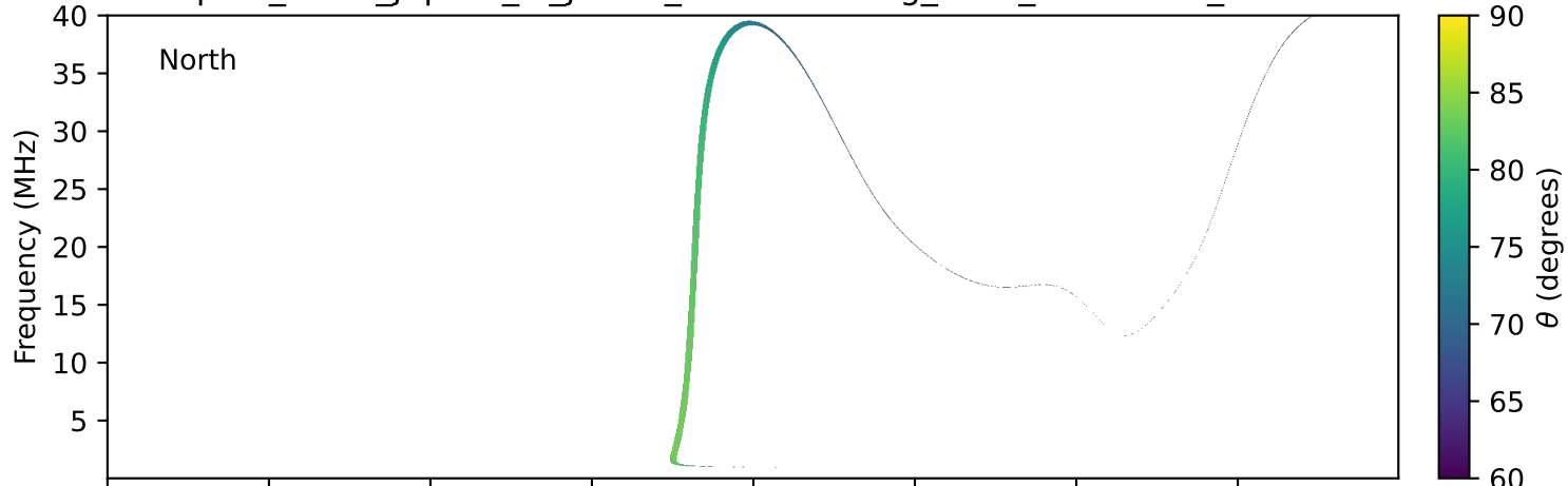
expres_earth_jupiter_io_jrm33_lossc-wid1deg_3kev_20261104_v11.cdf
