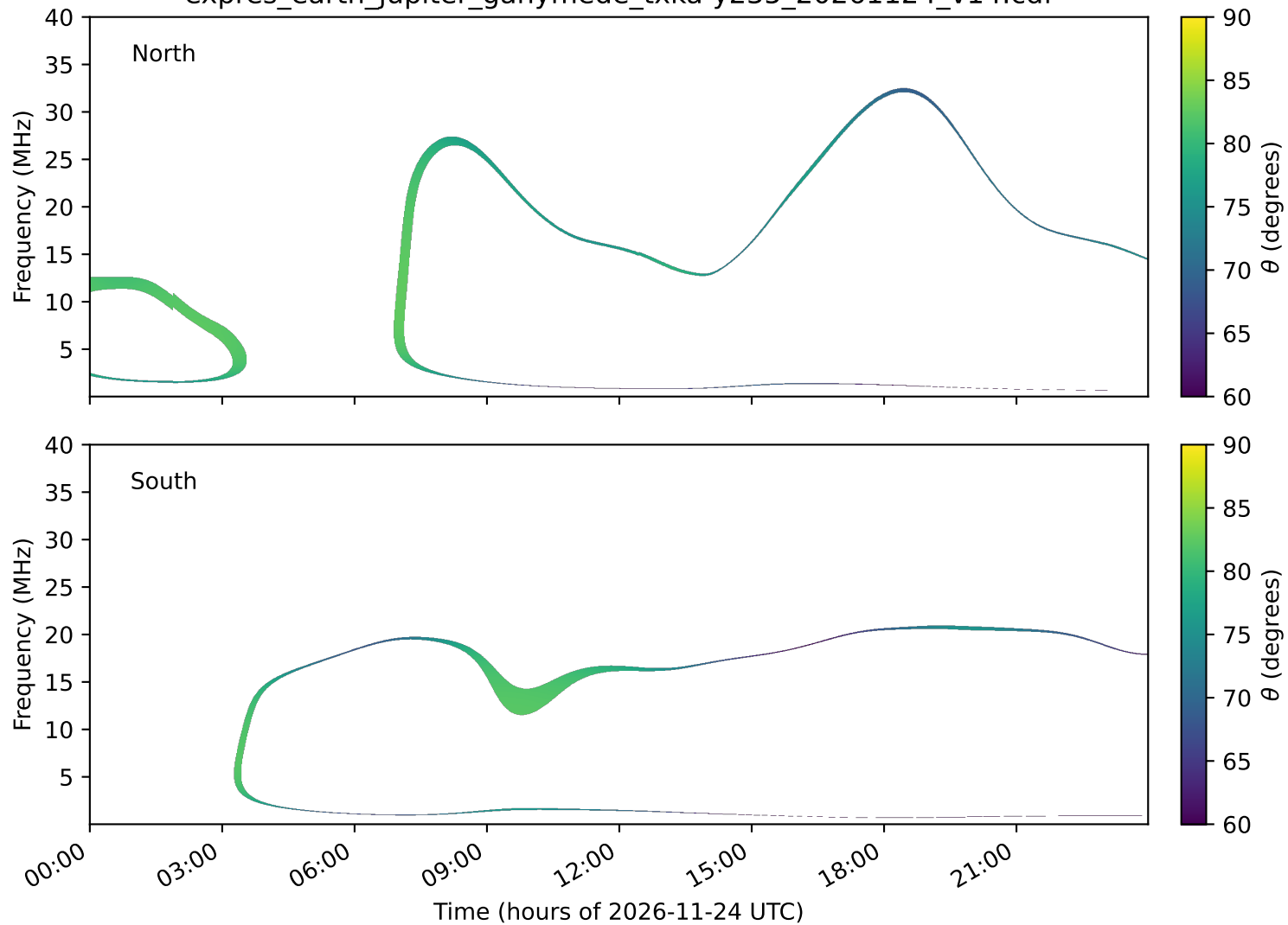
expres_earth_jupiter_ganymede_txka-y235_20261124_v14.cdf
