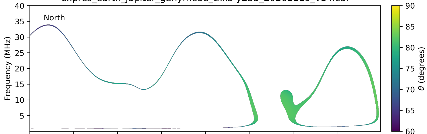
expres_earth_jupiter_ganymede_txka-y235_20261119_v14.cdf
