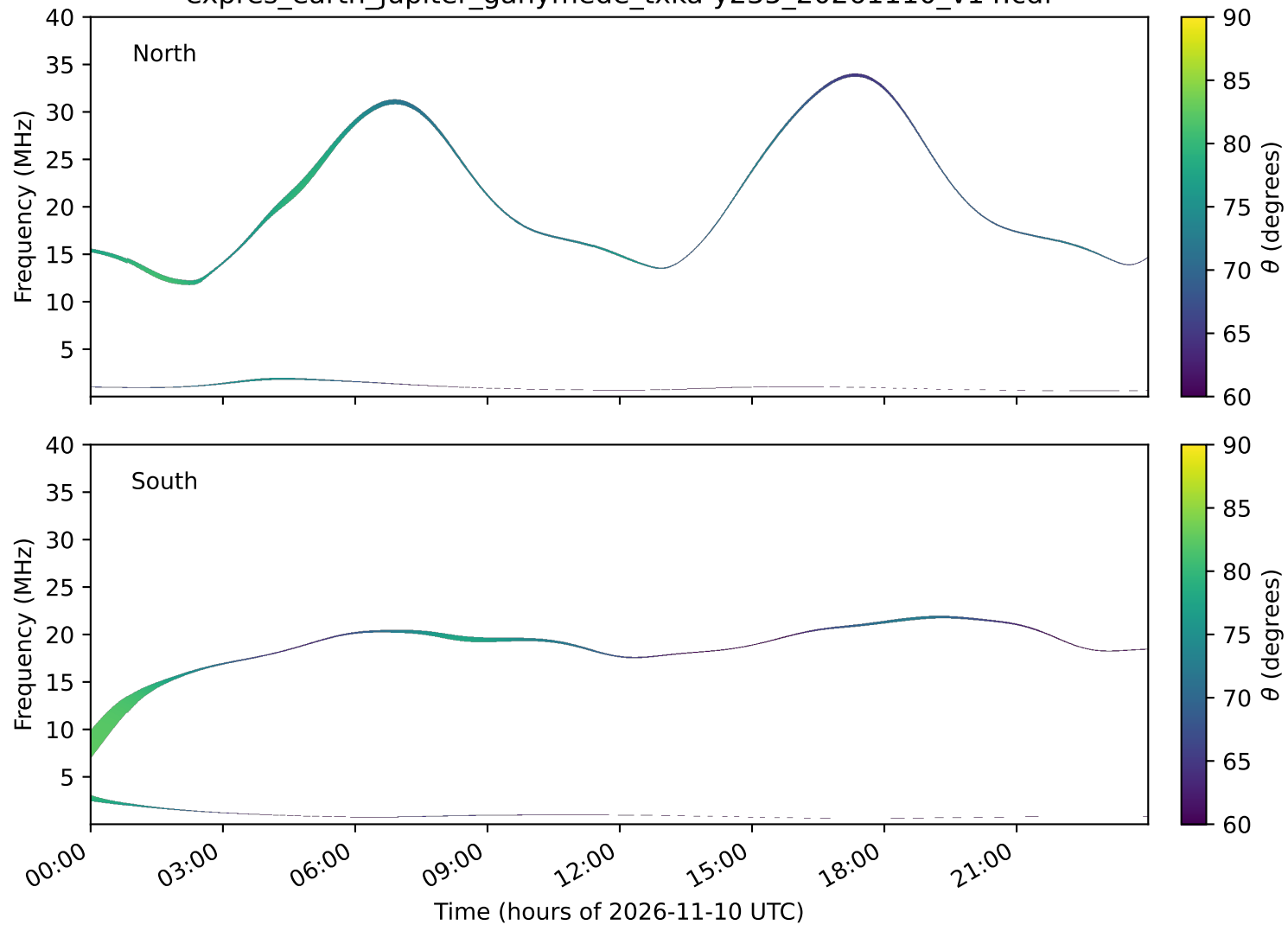
expres_earth_jupiter_ganymede_txka-y235_20261110_v14.cdf
