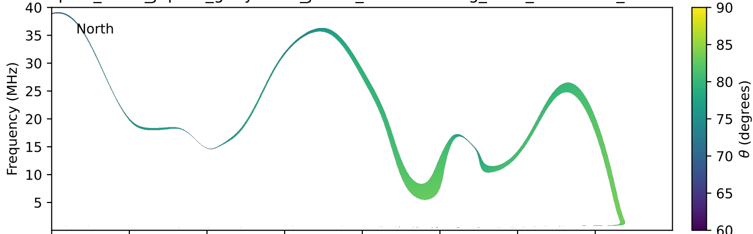
expres_earth_jupiter_ganymede_jrm33_lossc-wid1deg_3kev_20261105_v11.cdf
