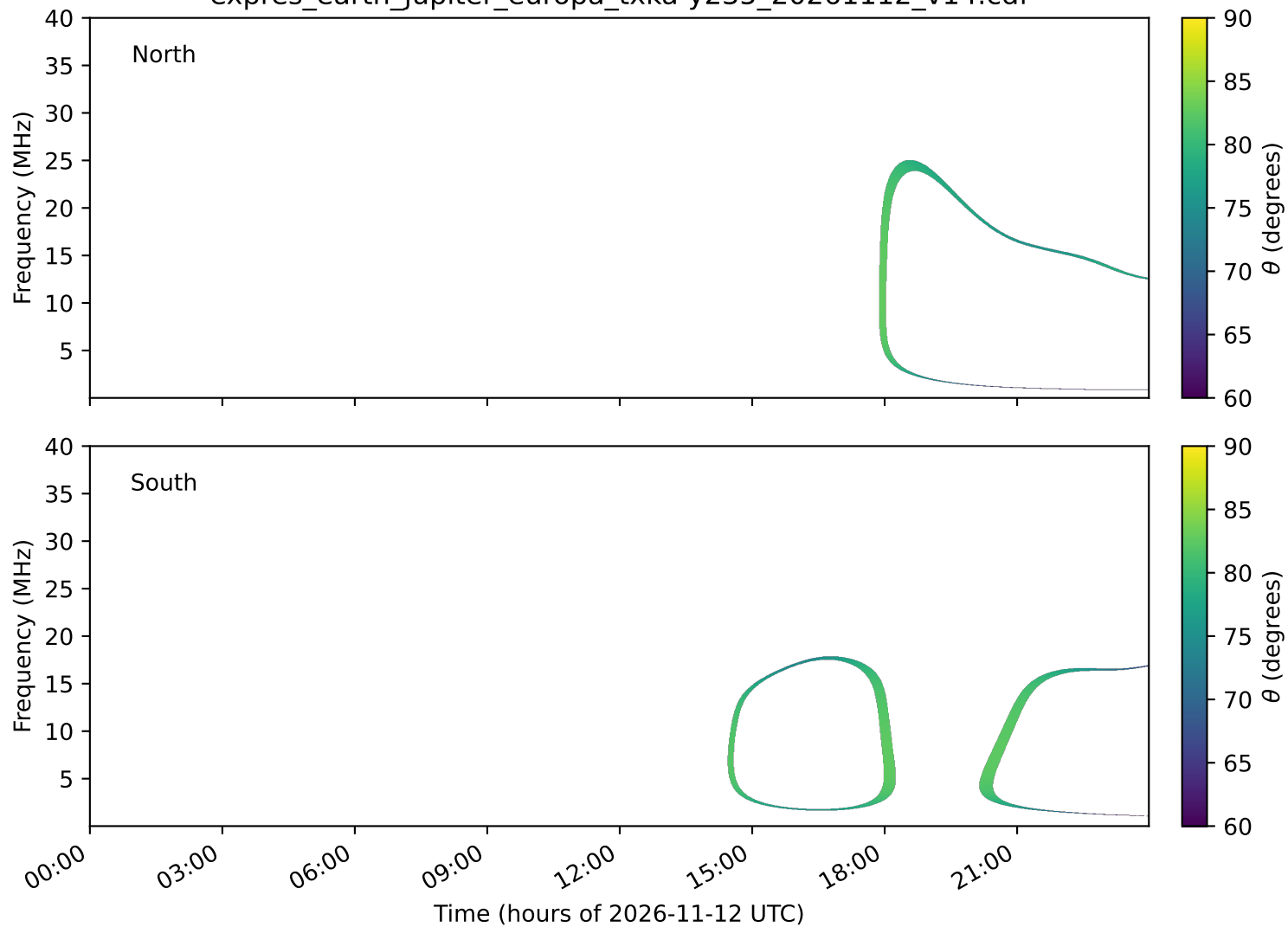
expres_earth_jupiter_europa_txka-y235_20261112_v14.cdf
