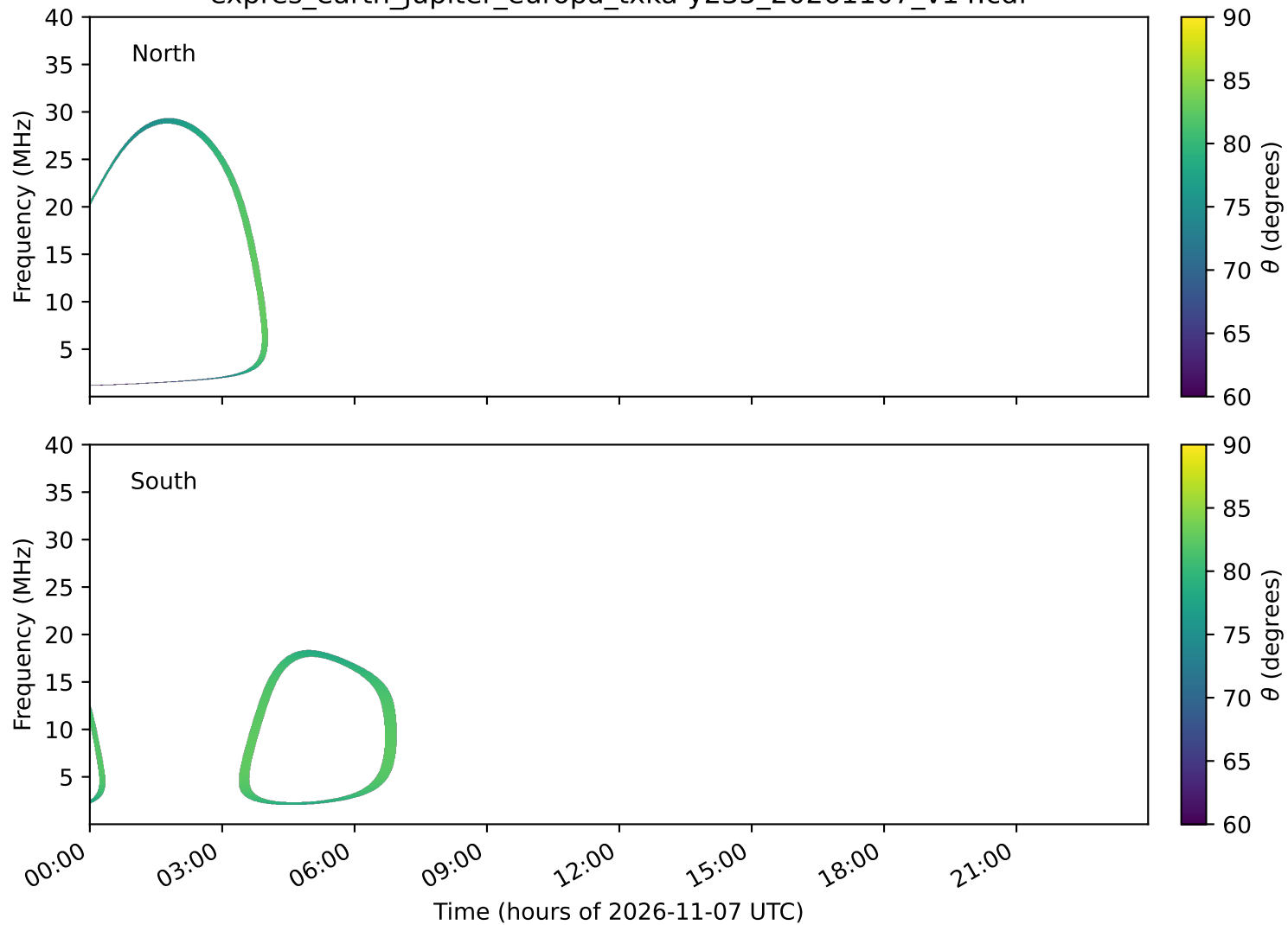
expres_earth_jupiter_europa_txka-y235_20261107_v14.cdf
