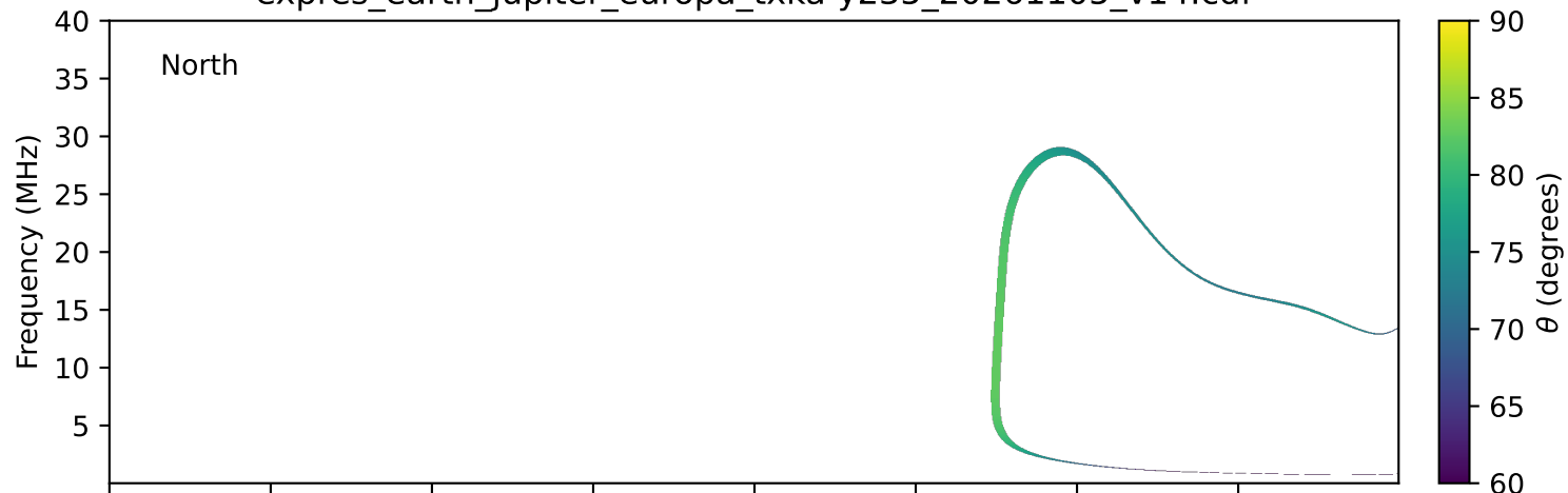
expres_earth_jupiter_europa_txka-y235_20261105_v14.cdf
