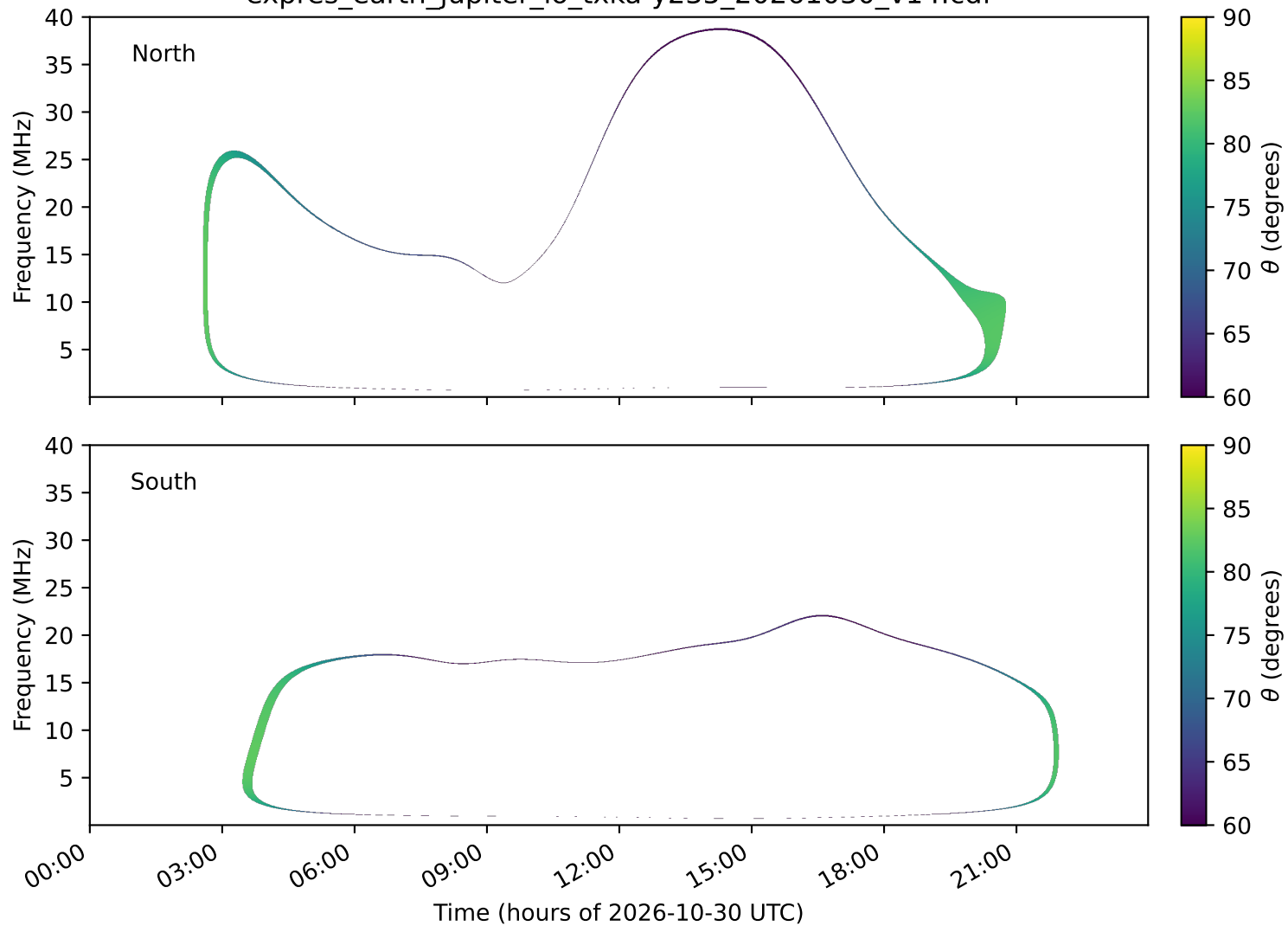
expres_earth_jupiter_io_txka-y235_20261030_v14.cdf
