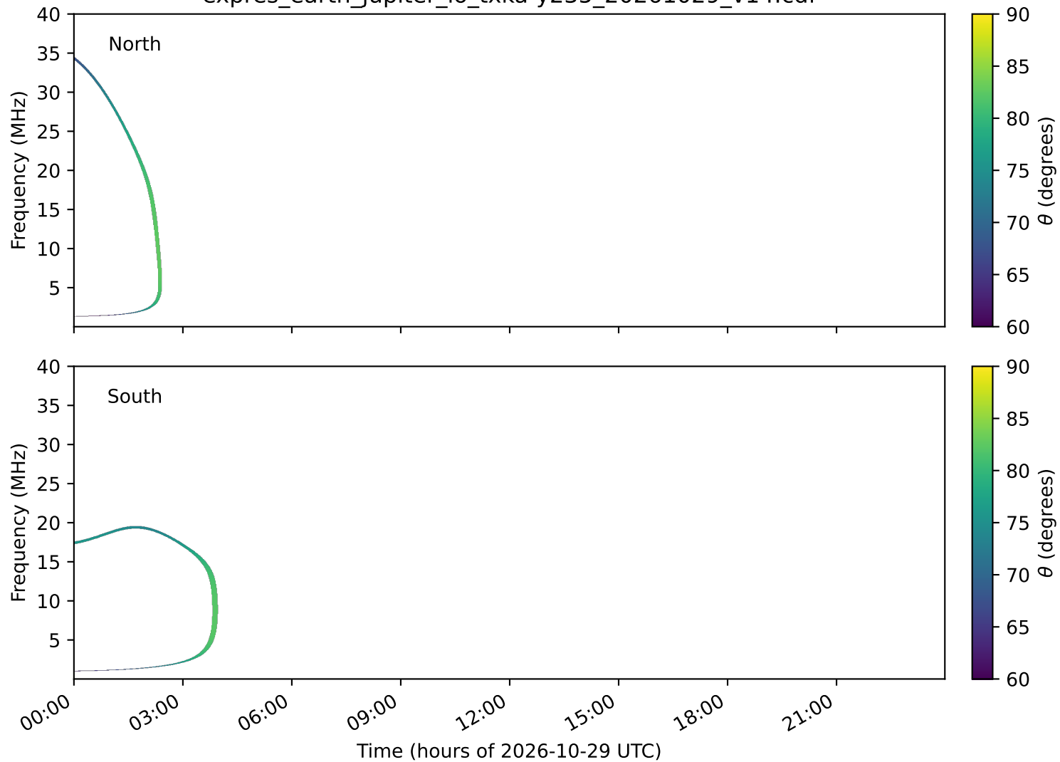
expres_earth_jupiter_io_txka-y235_20261029_v14.cdf
