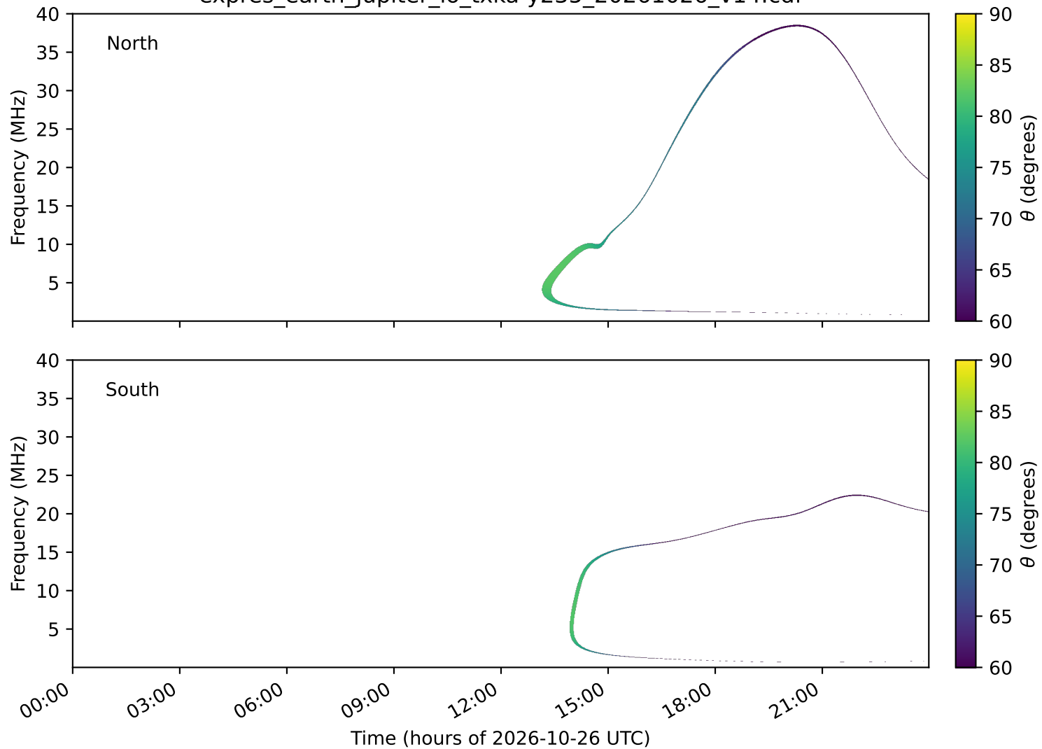
expres_earth_jupiter_io_txka-y235_20261026_v14.cdf
