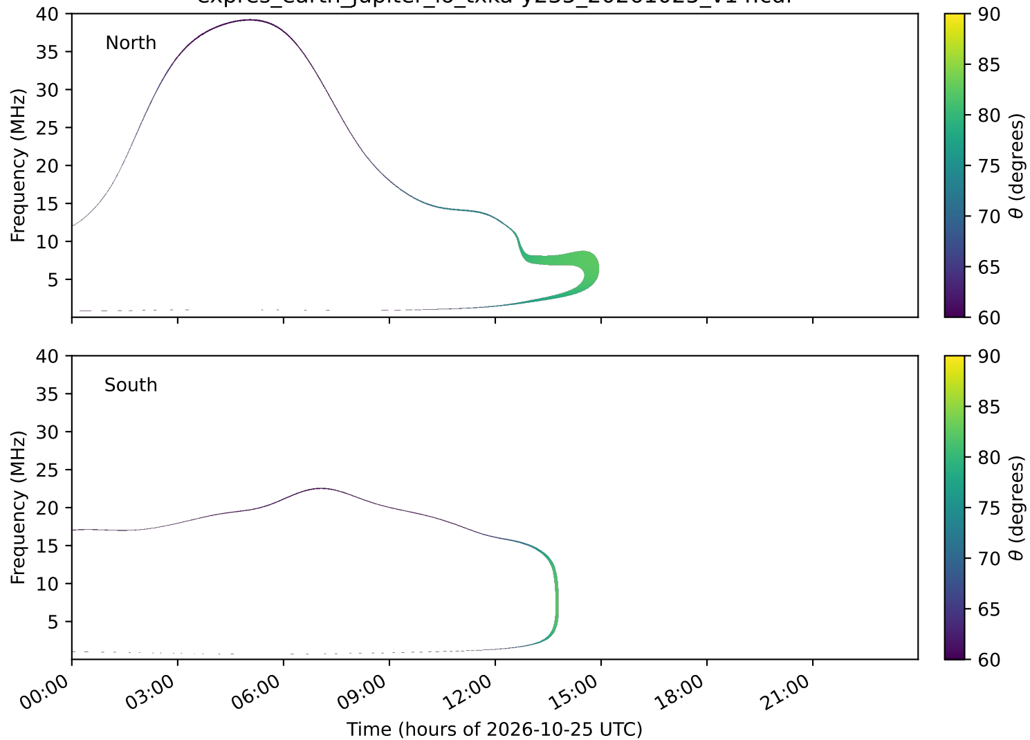
expres_earth_jupiter_io_txka-y235_20261025_v14.cdf
