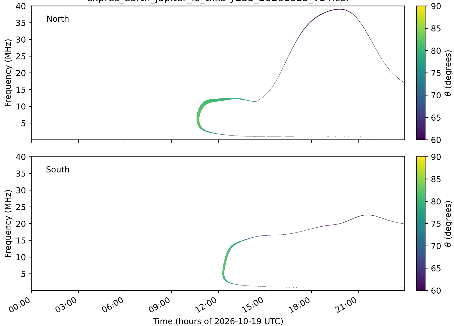
expres_earth_jupiter_io_txka-y235_20261019_v14.cdf
