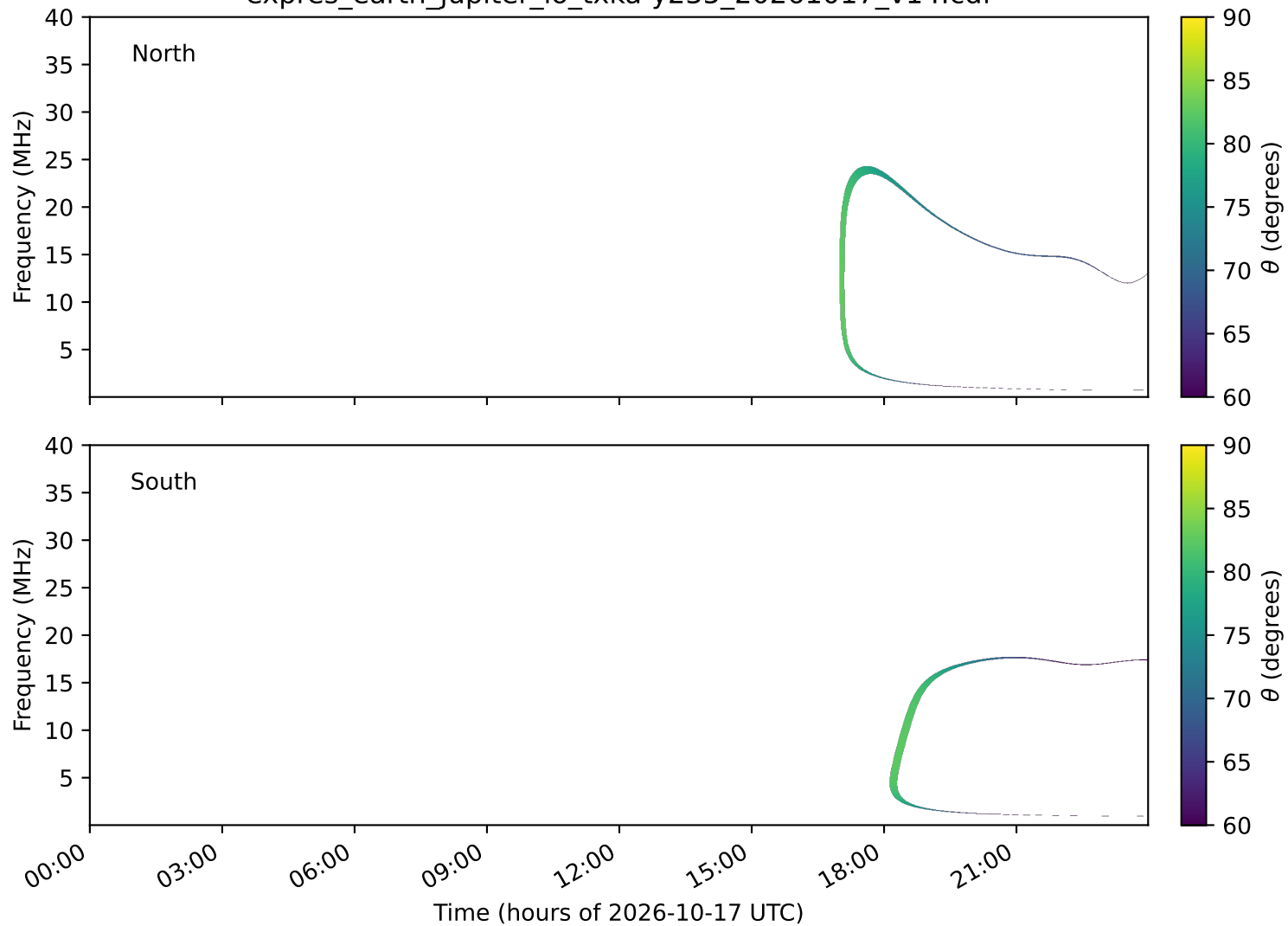
expres_earth_jupiter_io_txka-y235_20261017_v14.cdf
