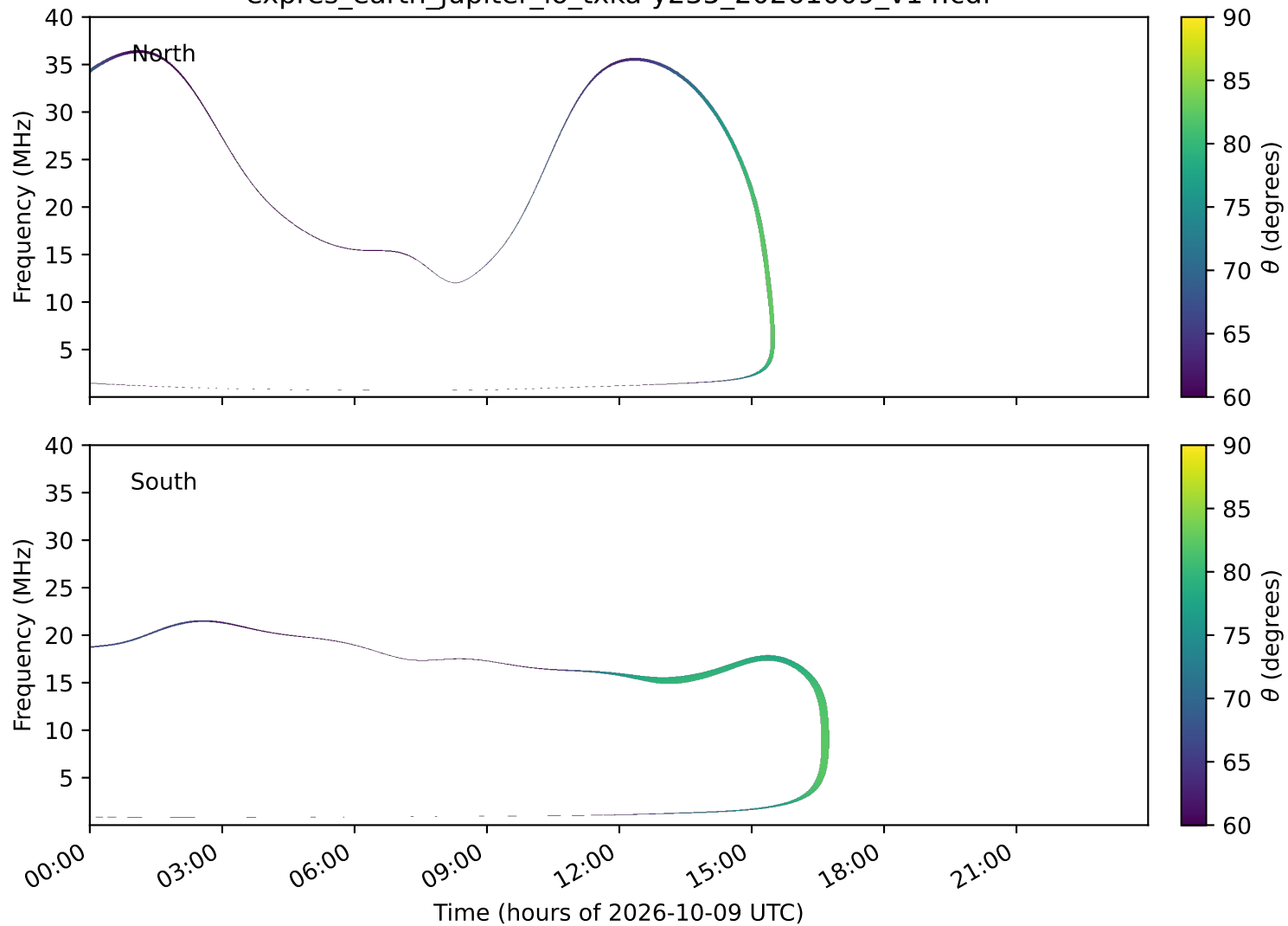
expres_earth_jupiter_io_txka-y235_20261009_v14.cdf
