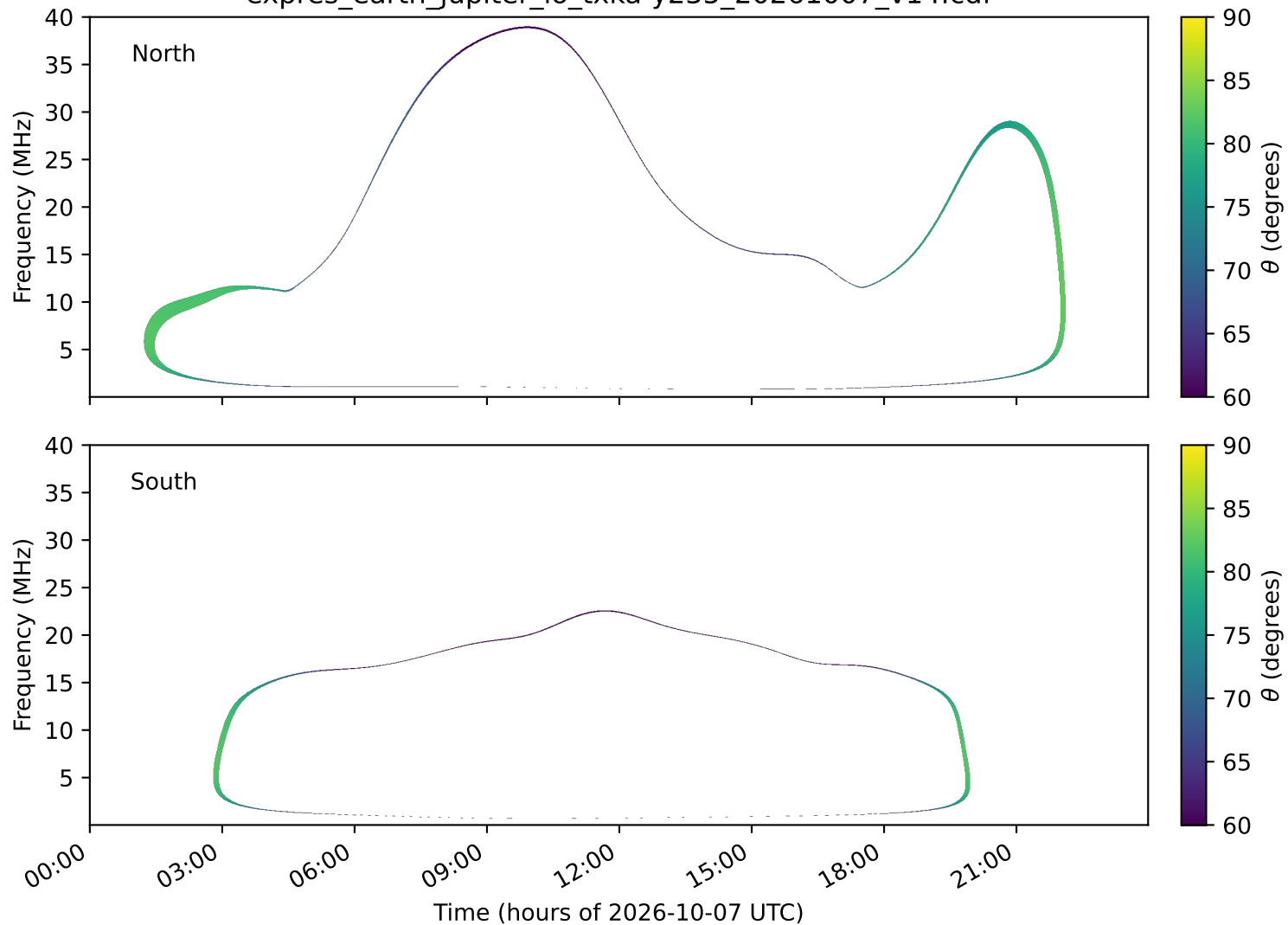
expres_earth_jupiter_io_txka-y235_20261007_v14.cdf
