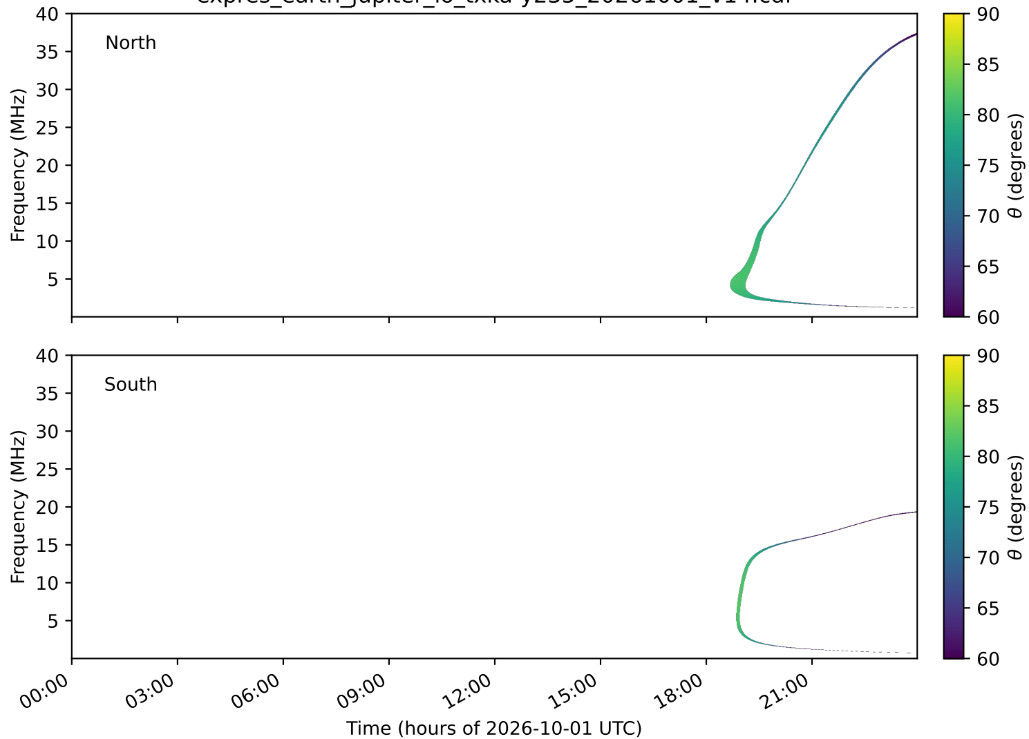
expres_earth_jupiter_io_txka-y235_20261001_v14.cdf
