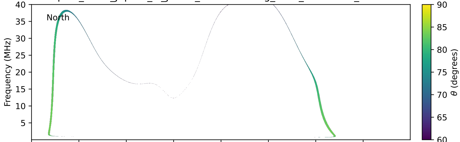
expres_earth_jupiter_io_jrm33_lossc-wid1deg_3kev_20261023_v11.cdf
