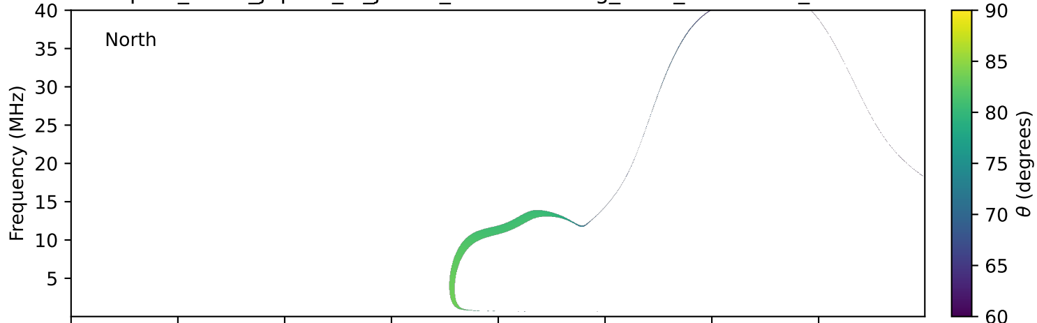
expres_earth_jupiter_io_jrm33_lossc-wid1deg_3kev_20261019_v11.cdf
