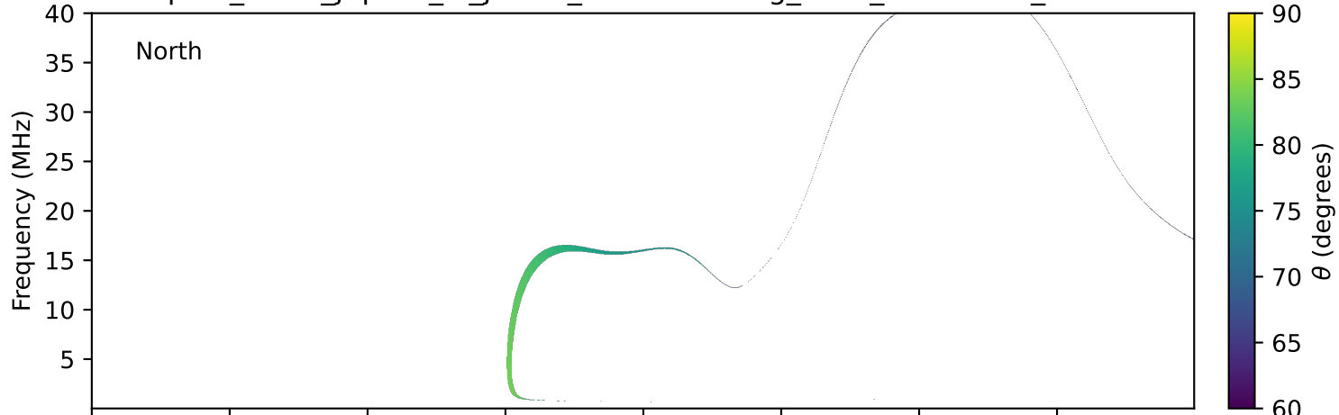
expres_earth_jupiter_io_jrm33_lossc-wid1deg_3kev_20261012_v11.cdf
