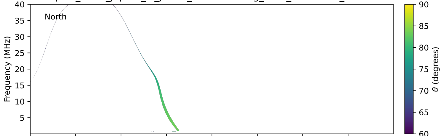
expres_earth_jupiter_io_jrm33_lossc-wid1deg_3kev_20261011_v11.cdf
