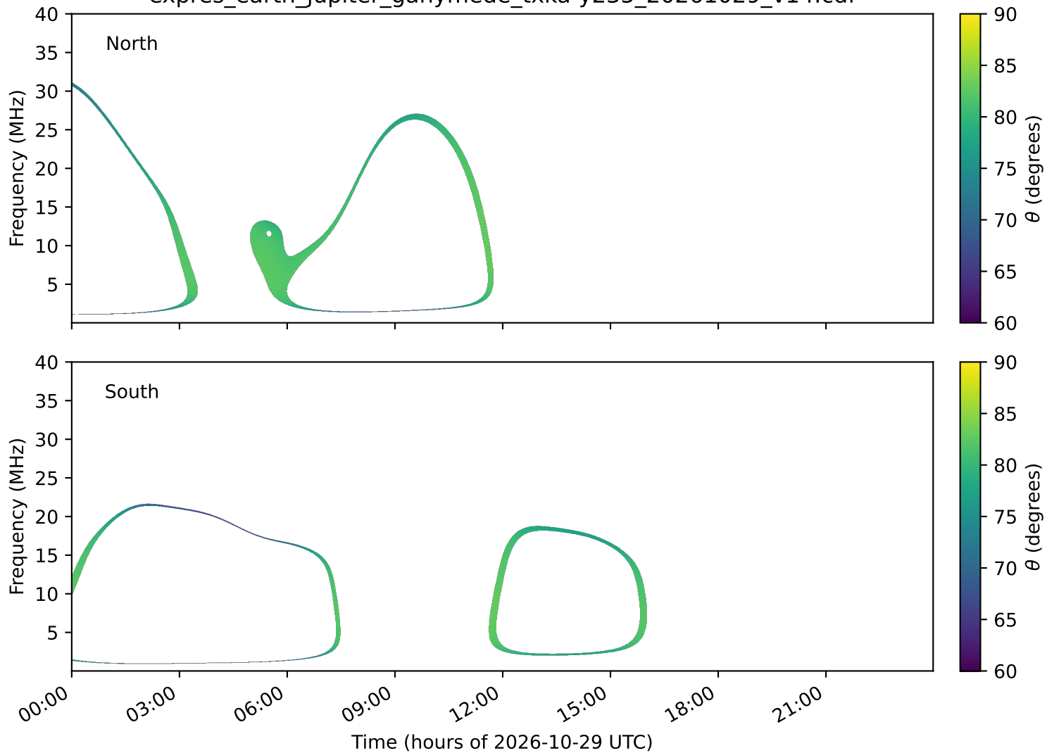
expres_earth_jupiter_ganymede_txka-y235_20261029_v14.cdf
