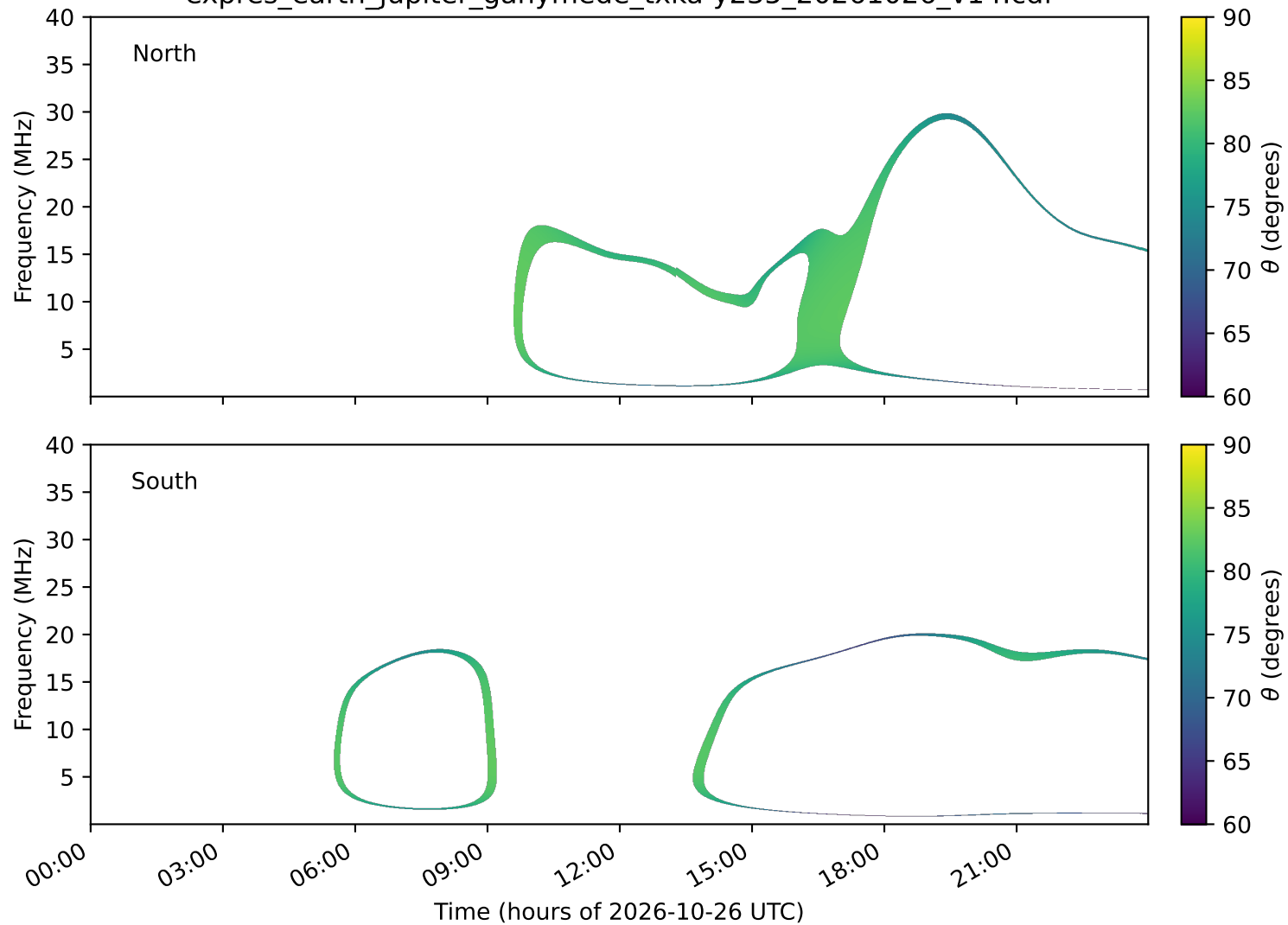
expres_earth_jupiter_ganymede_txka-y235_20261026_v14.cdf
