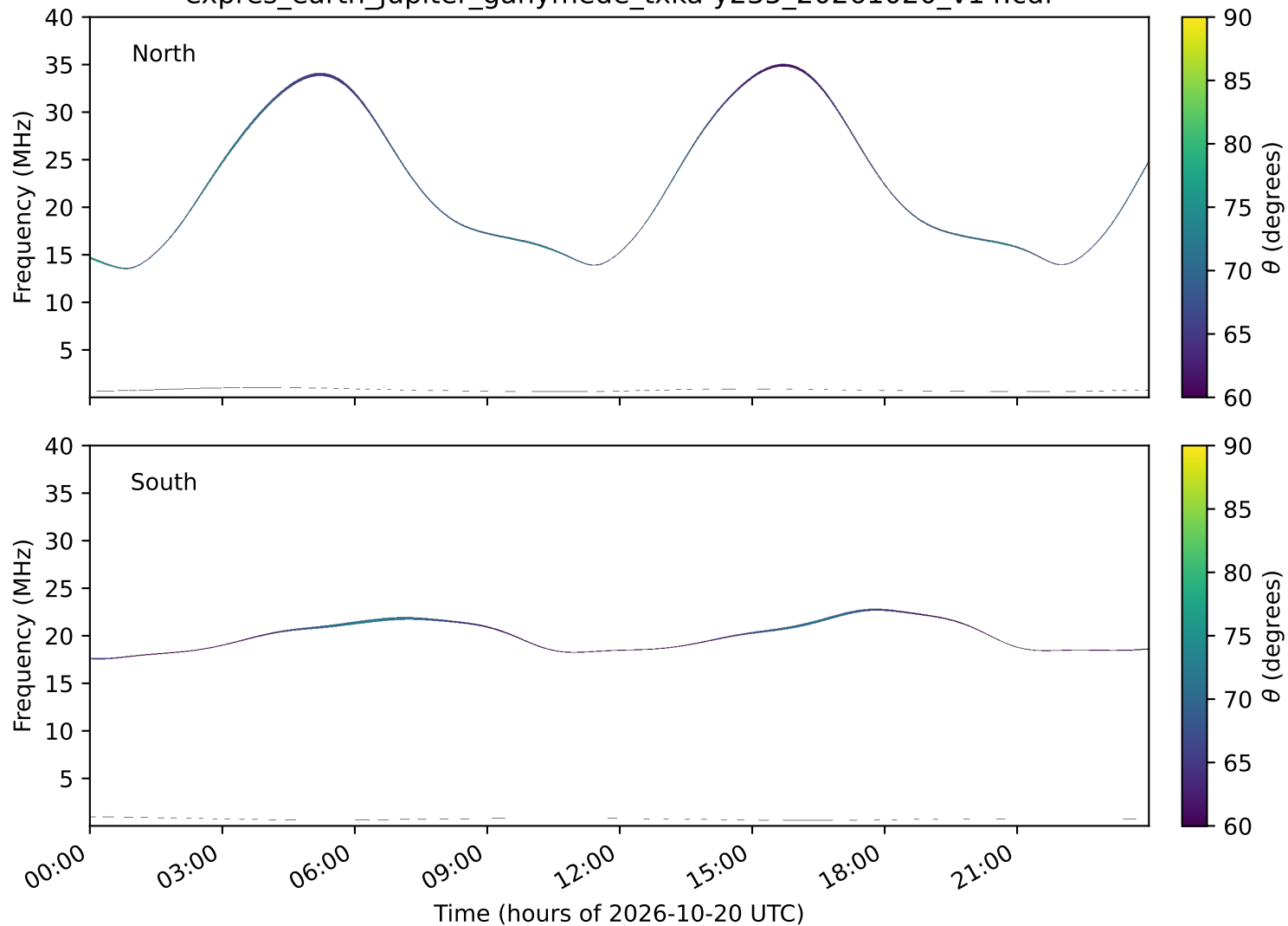
expres_earth_jupiter_ganymede_txka-y235_20261020_v14.cdf
