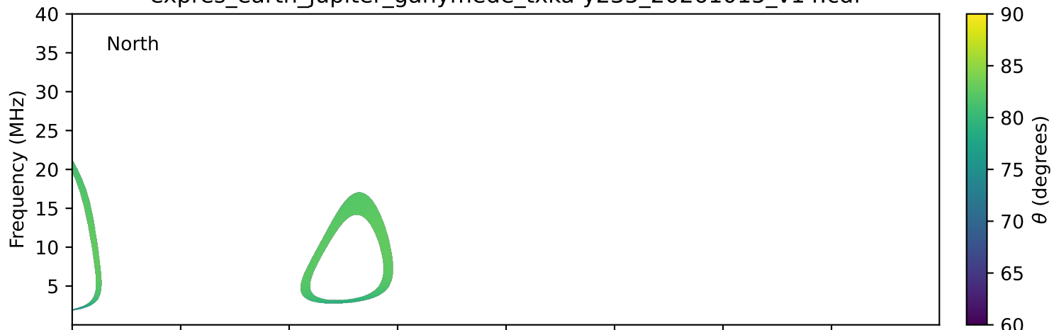
expres_earth_jupiter_ganymede_txka-y235_20261015_v14.cdf
