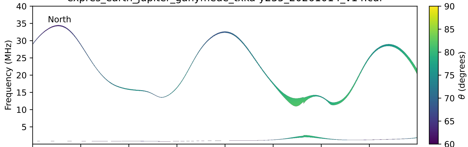
expres_earth_jupiter_ganymede_txka-y235_20261014_v14.cdf
