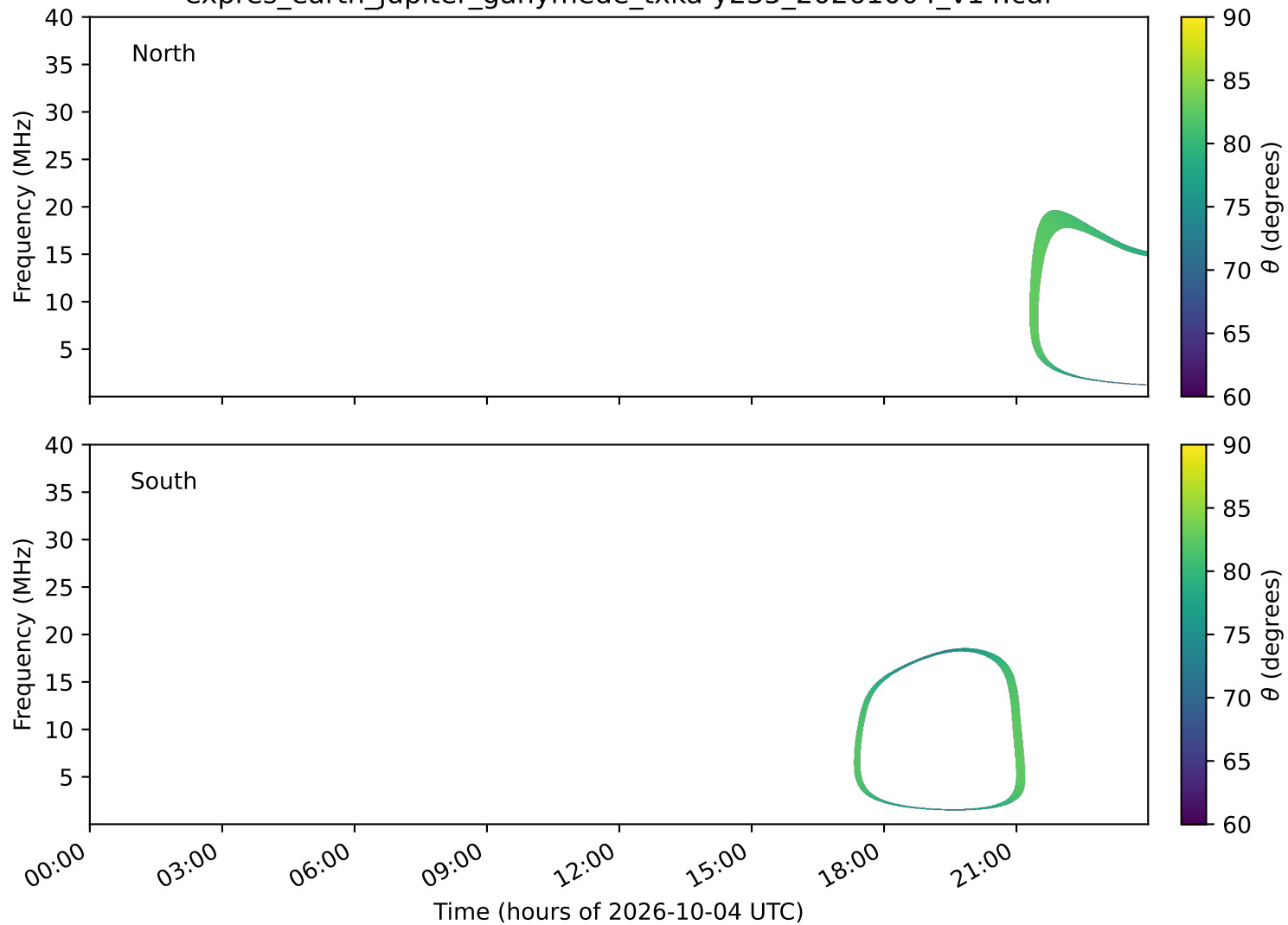
expres_earth_jupiter_ganymede_txka-y235_20261004_v14.cdf
