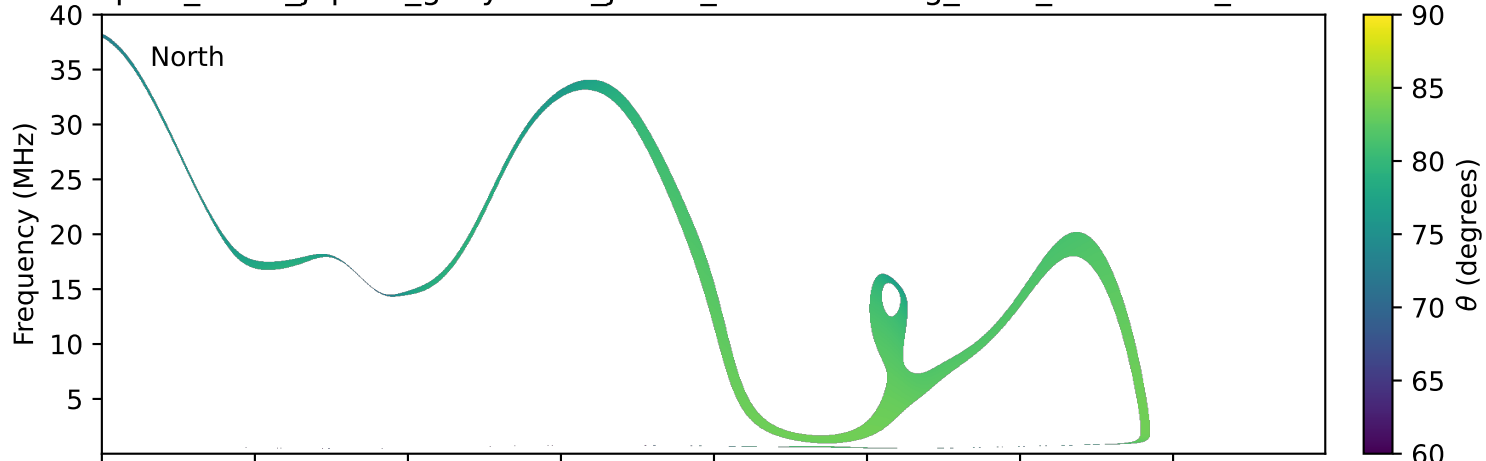
expres_earth_jupiter_ganymede_jrm33_lossc-wid1deg_3kev_20261029_v11.cdf
