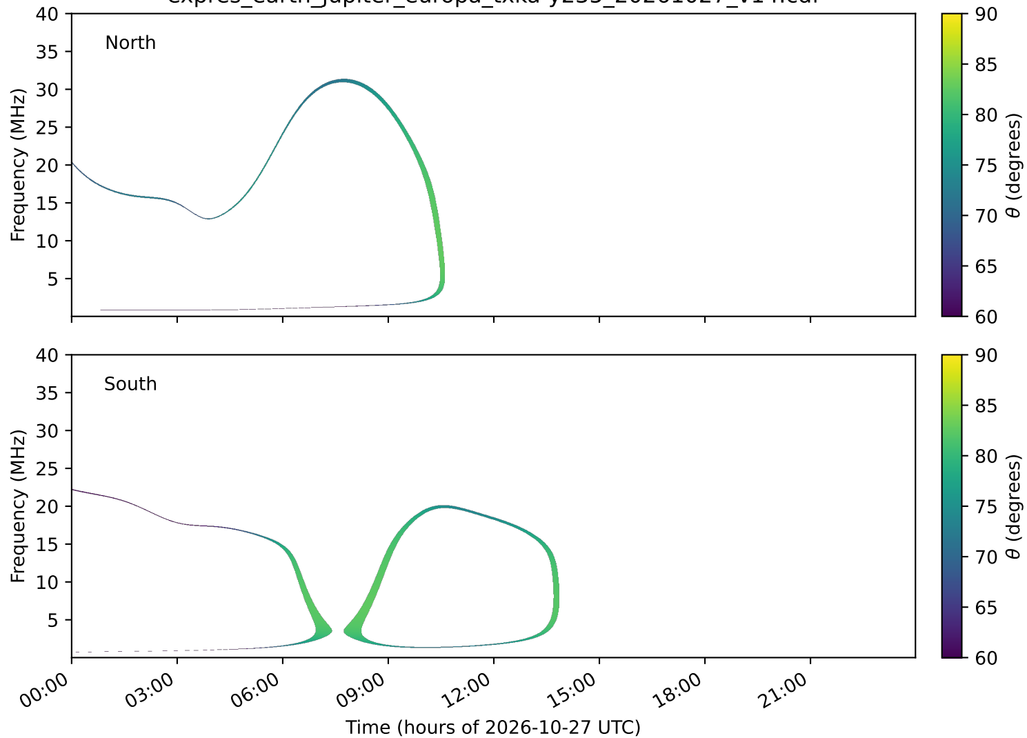
expres_earth_jupiter_europa_txka-y235_20261027_v14.cdf
