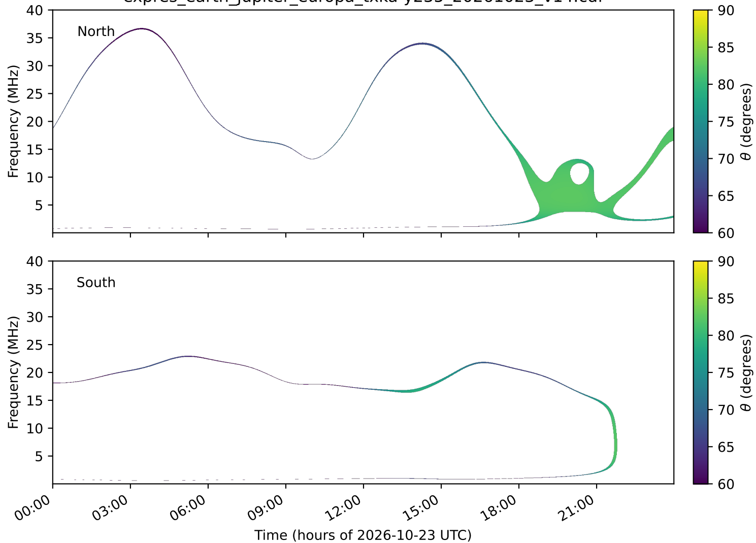
expres_earth_jupiter_europa_txka-y235_20261023_v14.cdf
