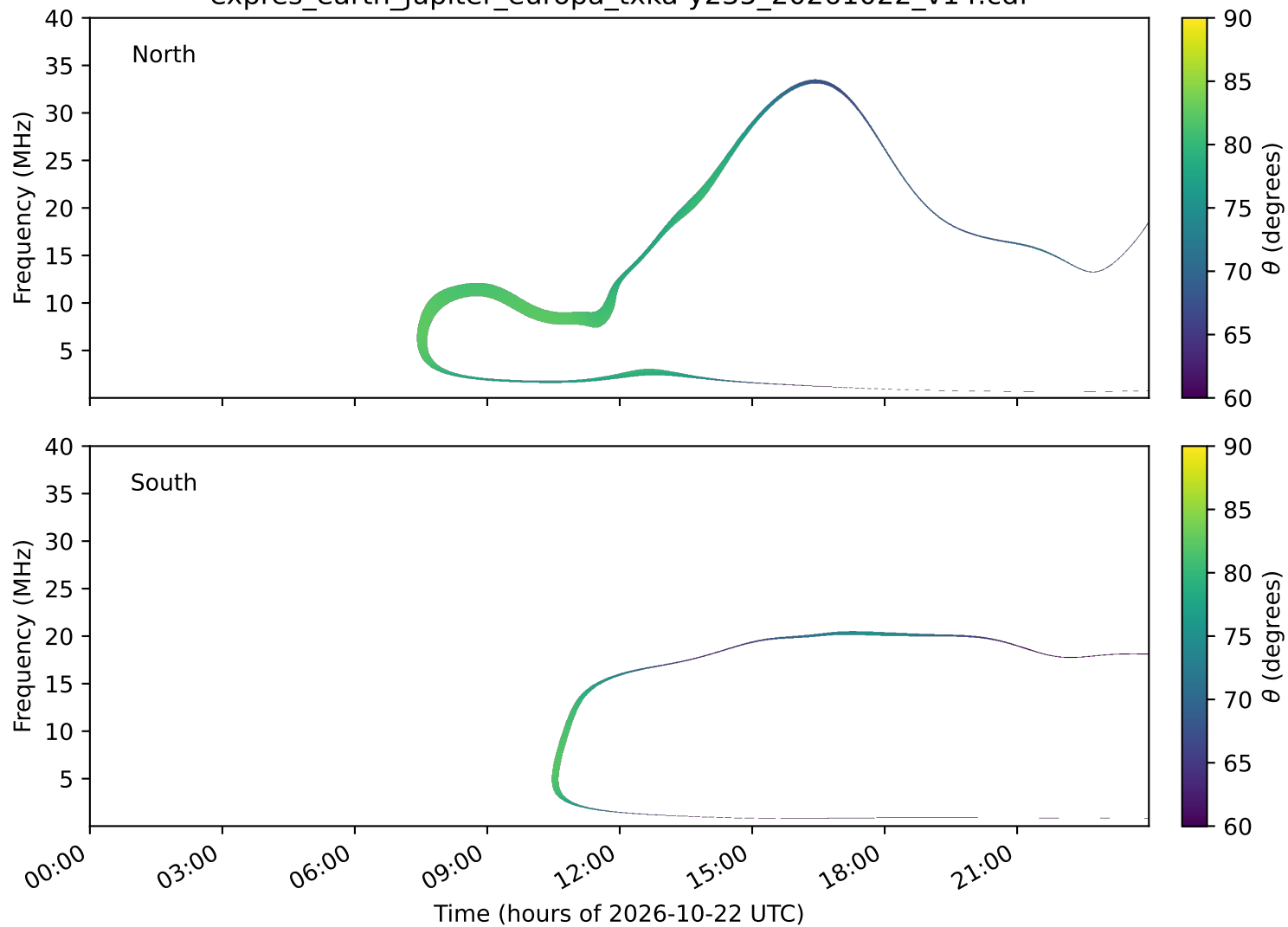
expres_earth_jupiter_europa_txka-y235_20261022_v14.cdf
