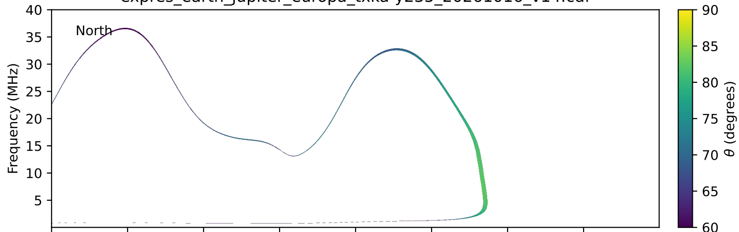
expres_earth_jupiter_europa_txka-y235_20261016_v14.cdf
