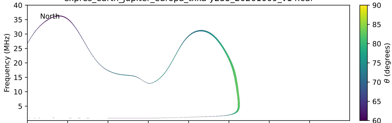
expres_earth_jupiter_europa_txka-y235_20261009_v14.cdf
