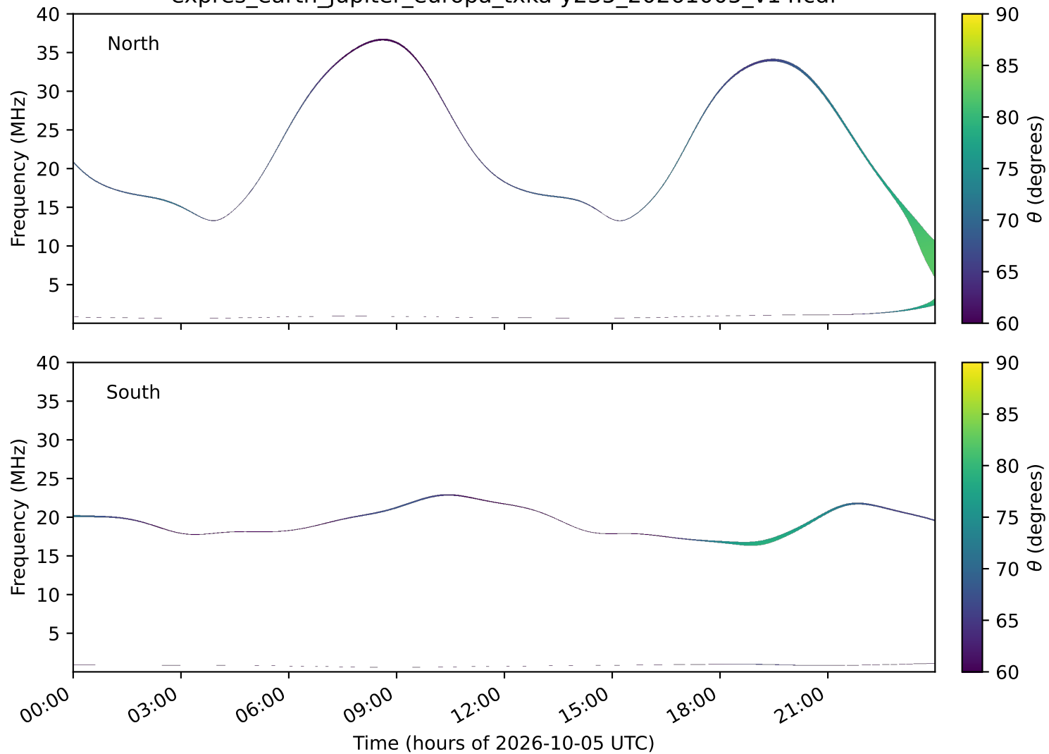
expres_earth_jupiter_europa_txka-y235_20261005_v14.cdf
