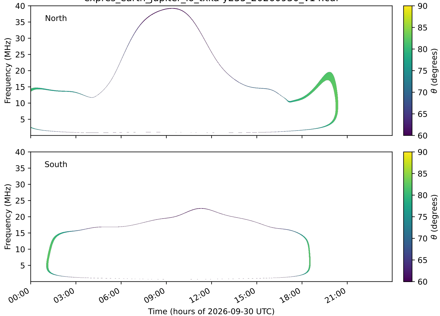
expres_earth_jupiter_io_txka-y235_20260930_v14.cdf
