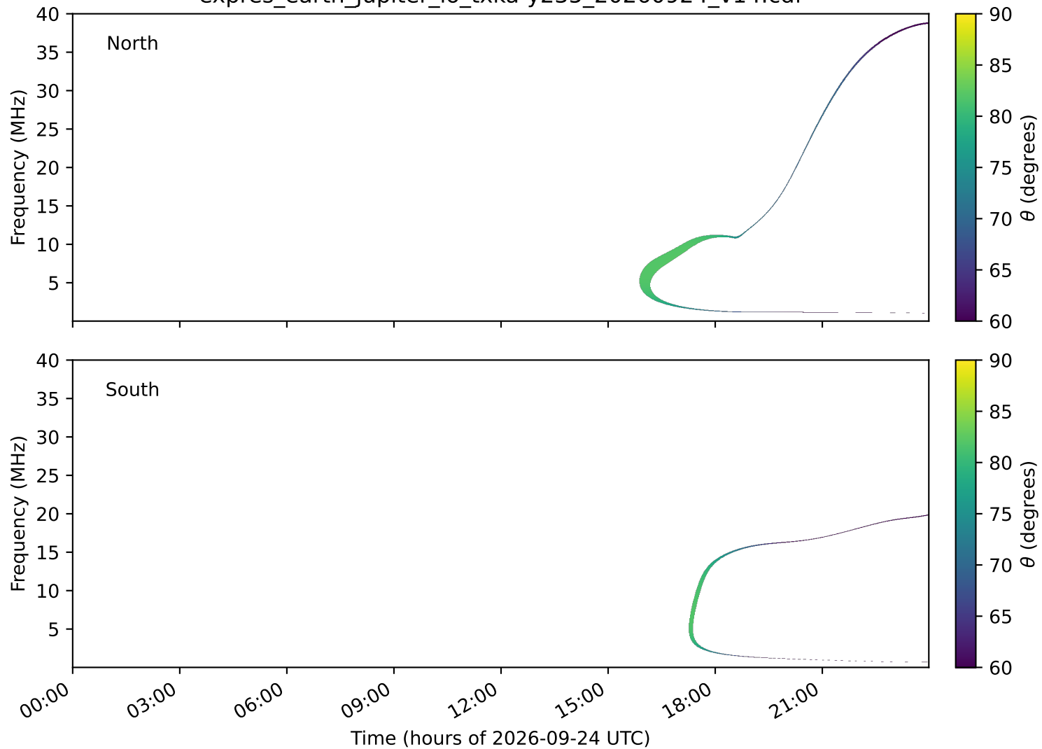
expres_earth_jupiter_io_txka-y235_20260924_v14.cdf
