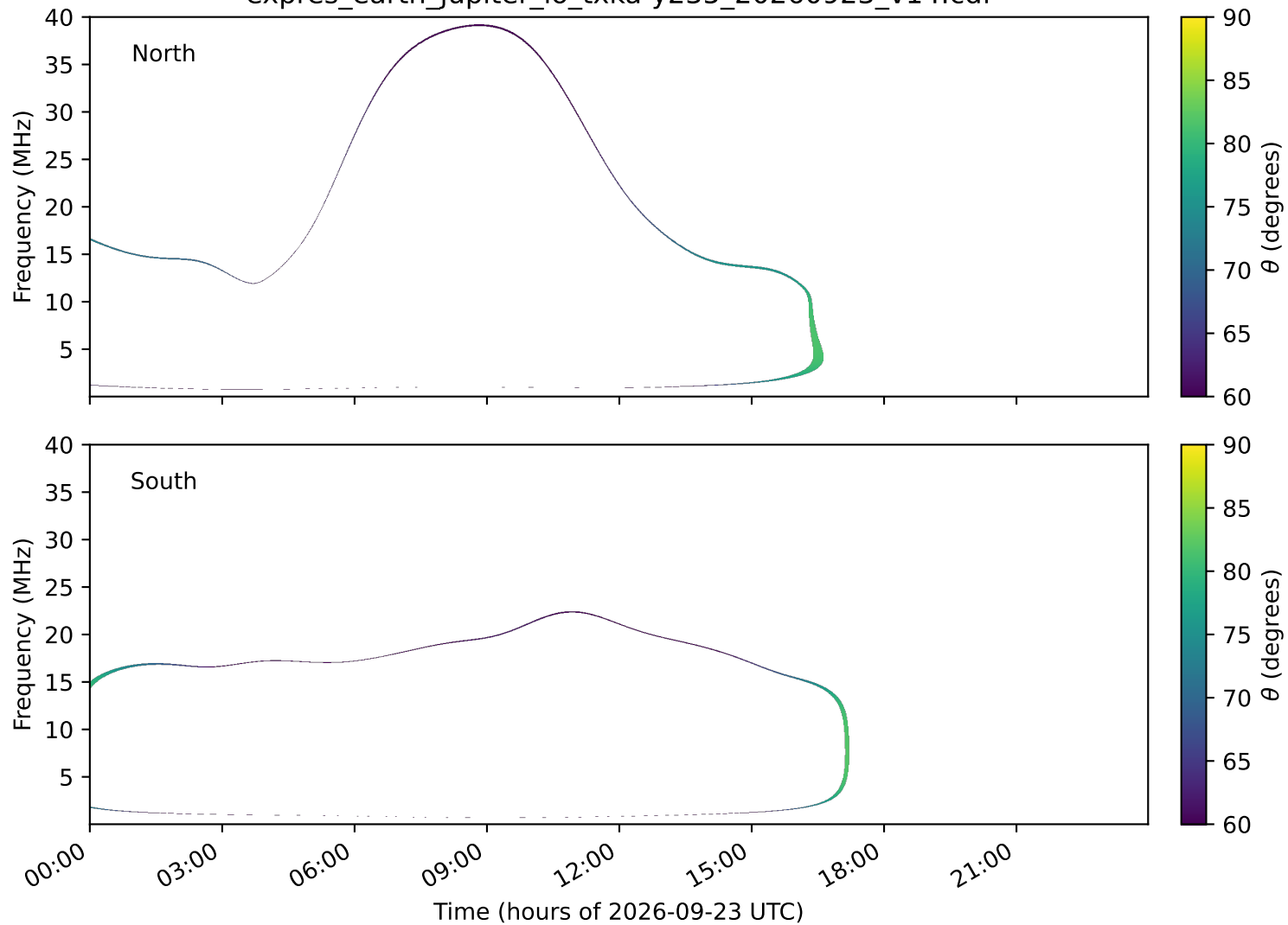
expres_earth_jupiter_io_txka-y235_20260923_v14.cdf
