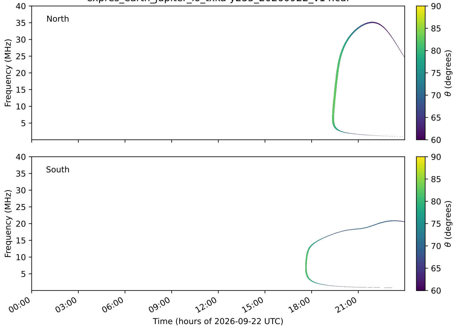
expres_earth_jupiter_io_txka-y235_20260922_v14.cdf
