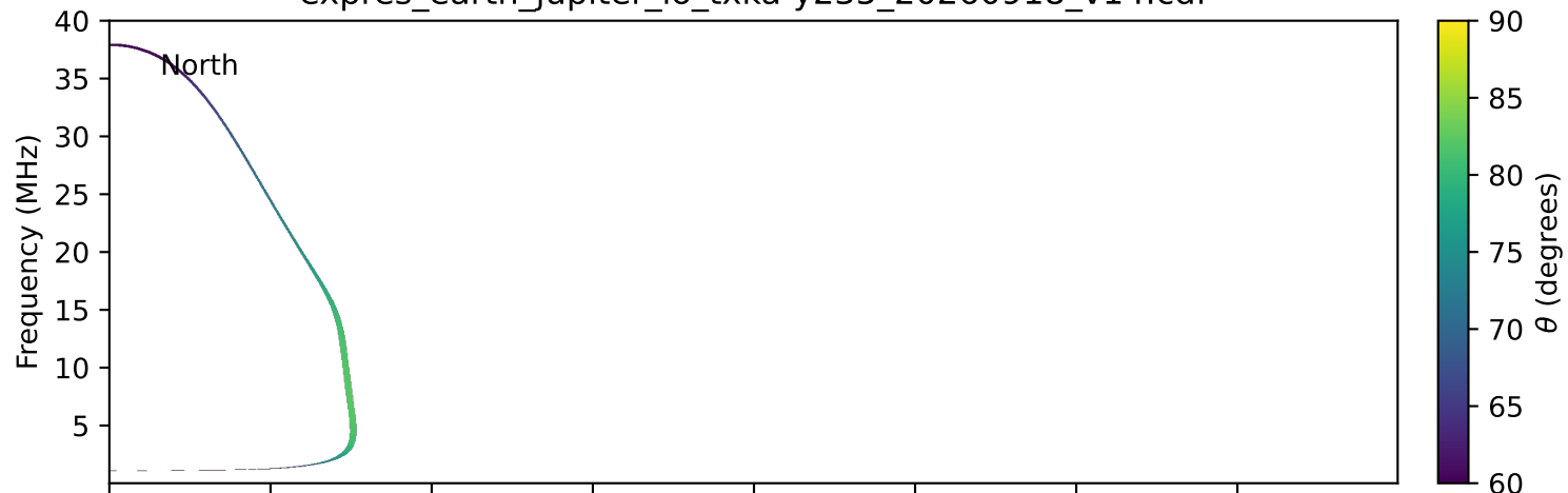
expres_earth_jupiter_io_txka-y235_20260918_v14.cdf
