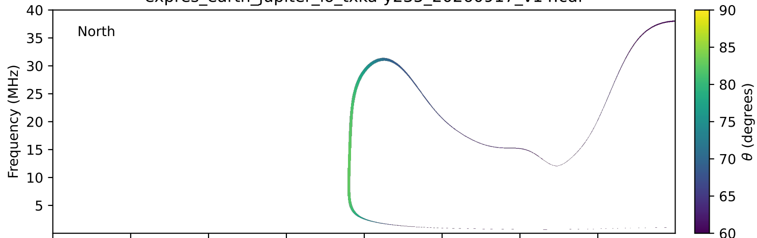
expres_earth_jupiter_io_txka-y235_20260917_v14.cdf
