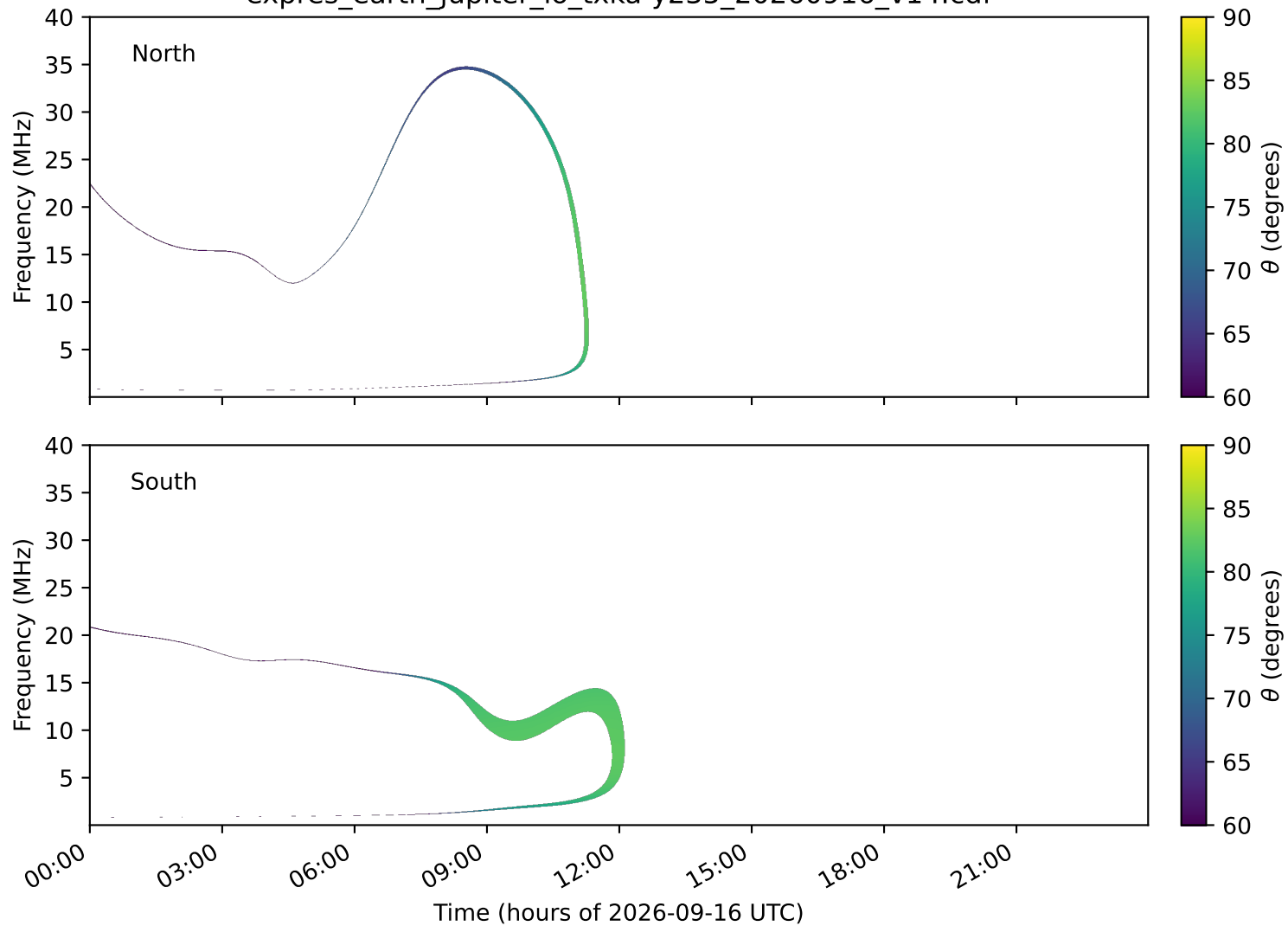
expres_earth_jupiter_io_txka-y235_20260916_v14.cdf
