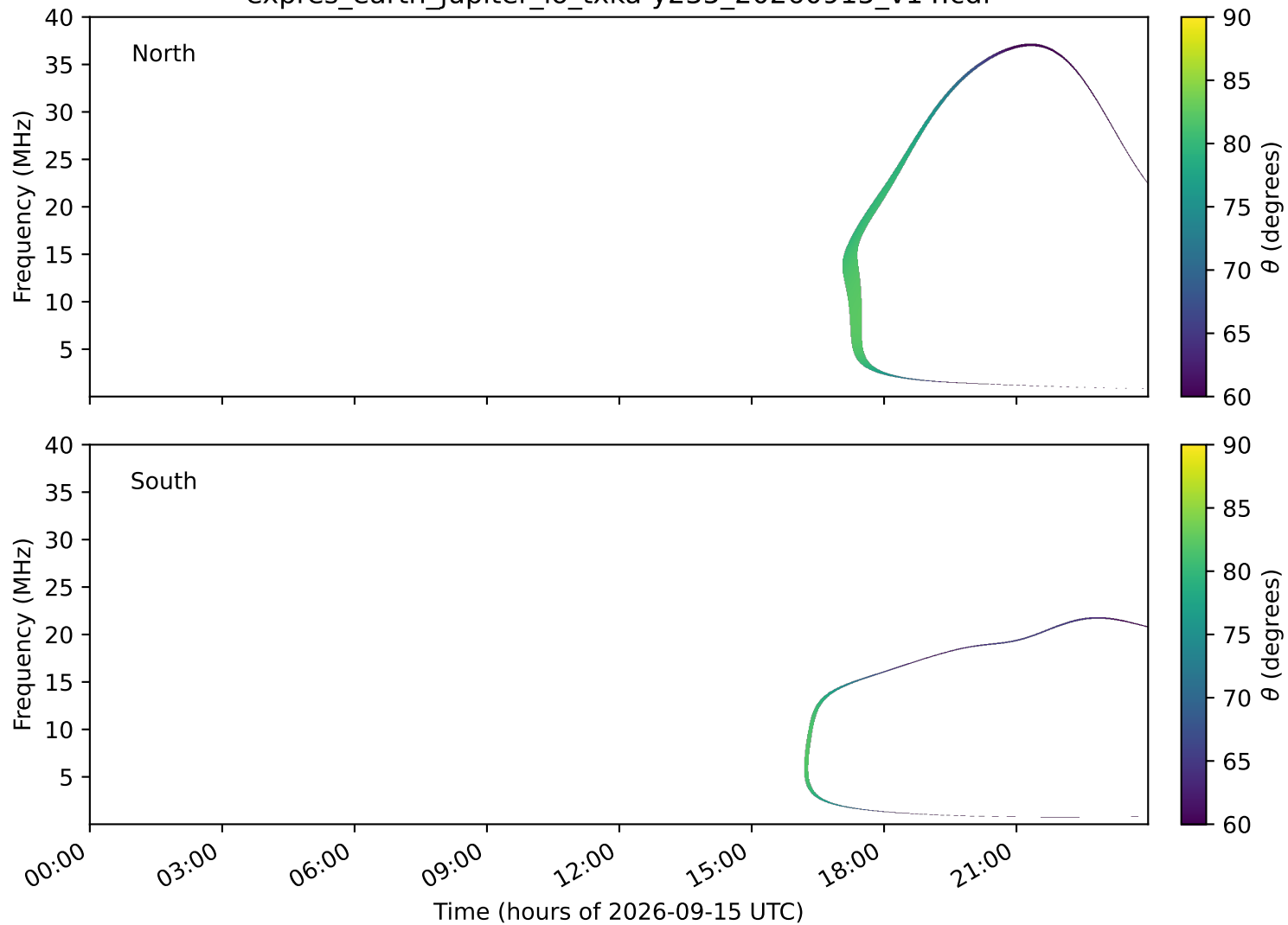
expres_earth_jupiter_io_txka-y235_20260915_v14.cdf
