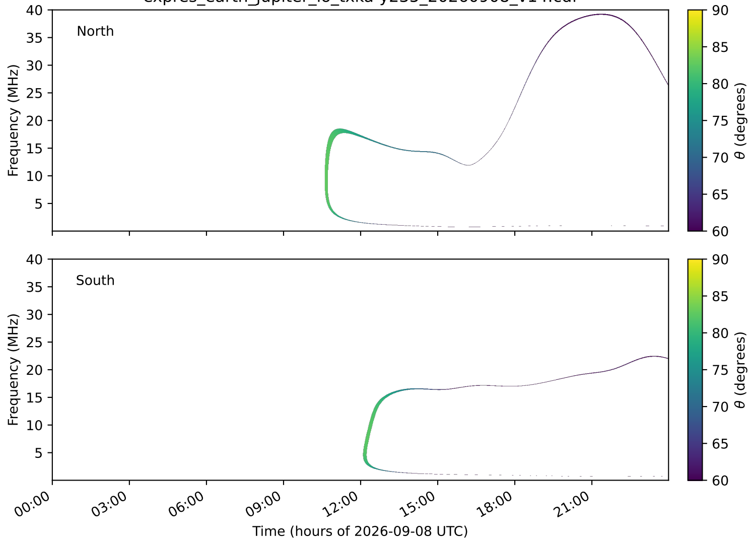
expres_earth_jupiter_io_txka-y235_20260908_v14.cdf
