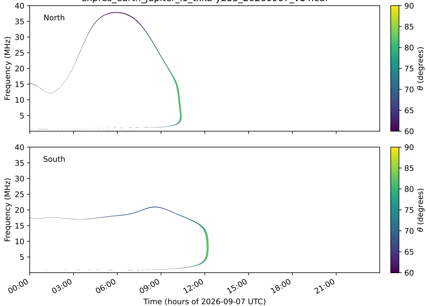
expres_earth_jupiter_io_txka-y235_20260907_v14.cdf
