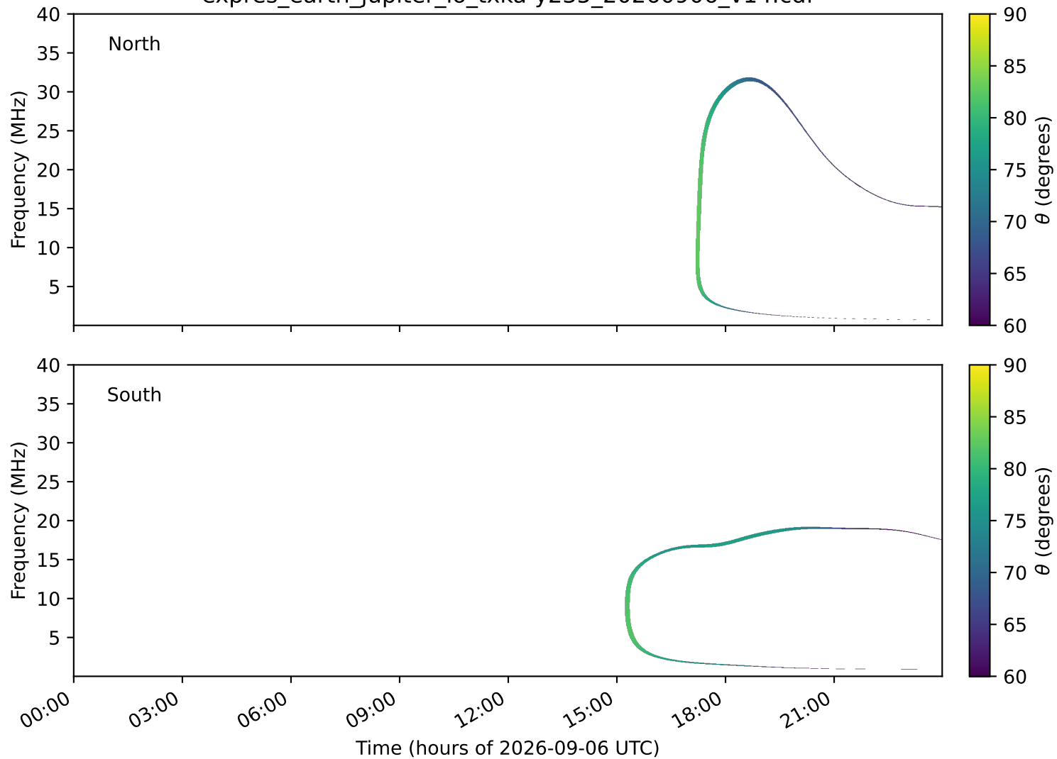
expres_earth_jupiter_io_txka-y235_20260906_v14.cdf
