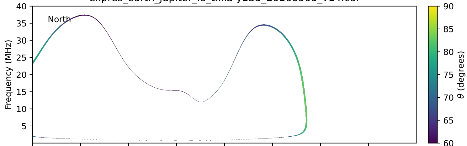
expres_earth_jupiter_io_txka-y235_20260905_v14.cdf
