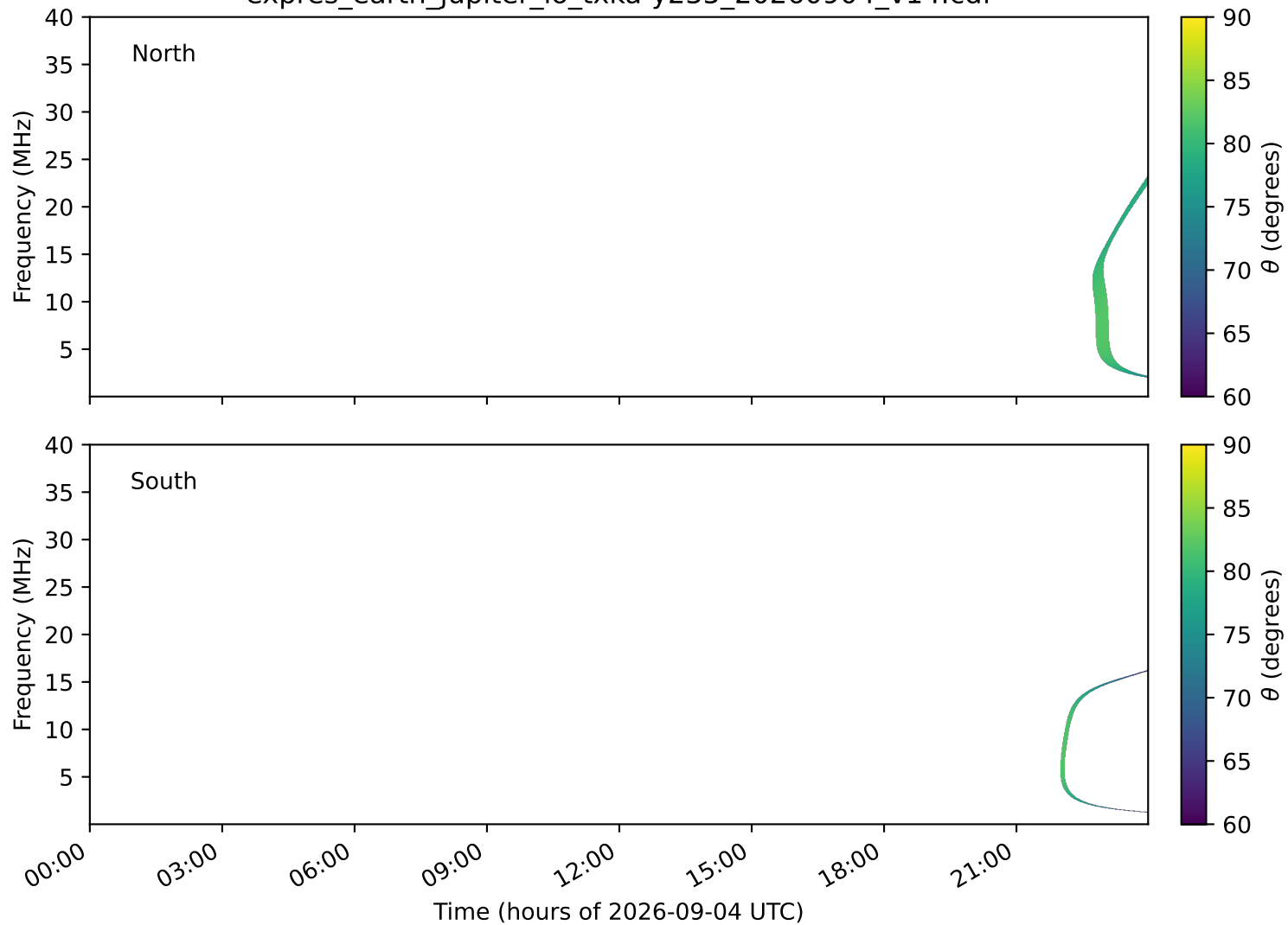
expres_earth_jupiter_io_txka-y235_20260904_v14.cdf
