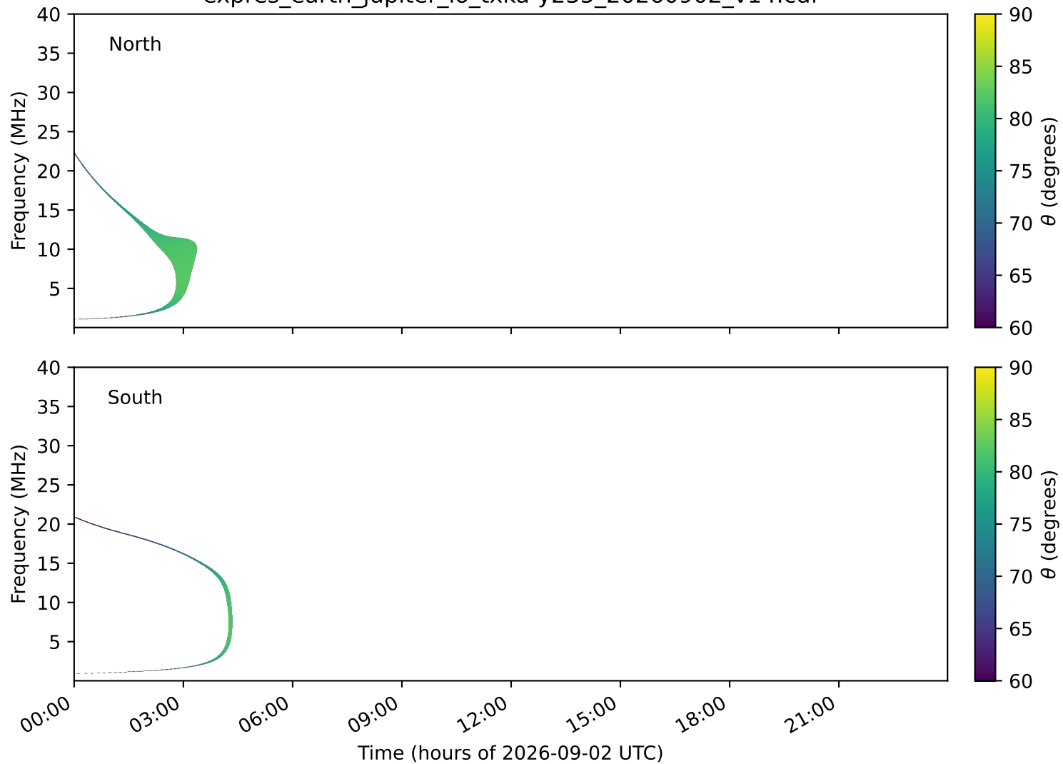
expres_earth_jupiter_io_txka-y235_20260902_v14.cdf
